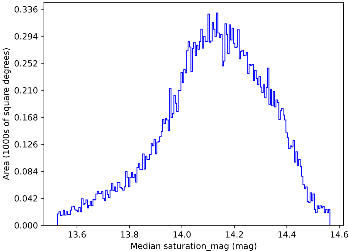
too_100_1v3.4_10yrs All sky all bands: Median saturation_mag
