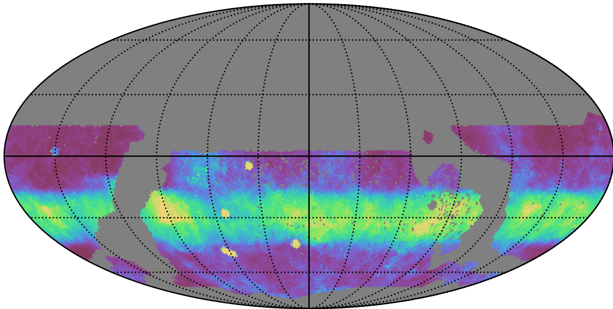
too_100_1v3.4_10yrs WFD z band: Median normairmass
