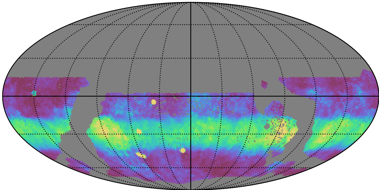
too_100_1v3.4_10yrs WFD y band: Median normairmass
