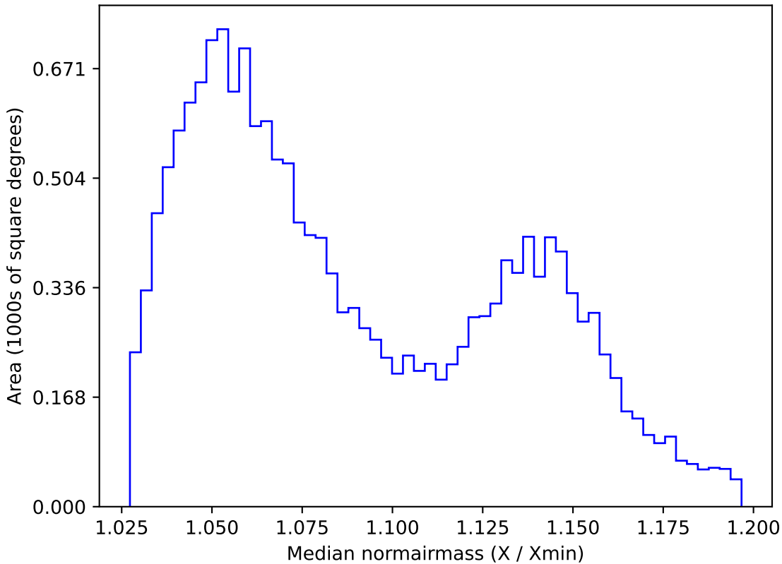
too_100_1v3.4_10yrs WFD y band: Median normairmass
