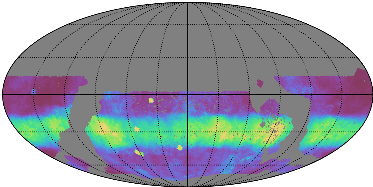
too_100_1v3.4_10yrs WFD r band: Median normairmass
