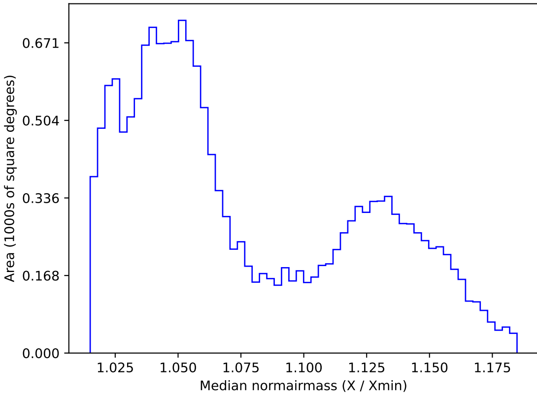
too_100_1v3.4_10yrs WFD r band: Median normairmass
