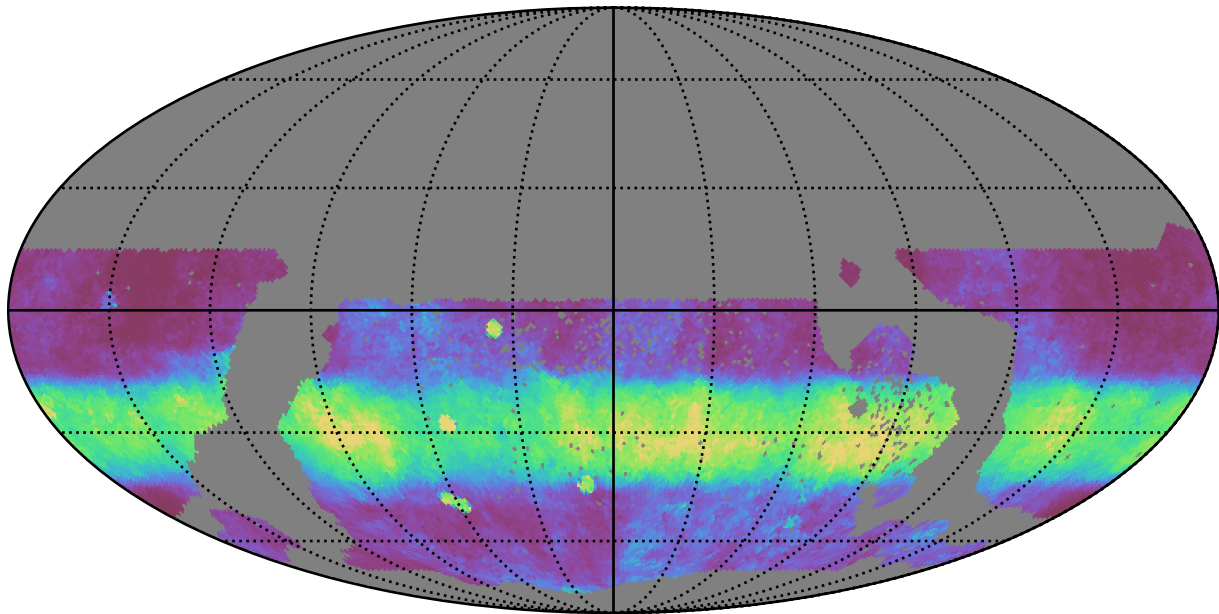
too_100_1v3.4_10yrs WFD i band: Median normairmass
