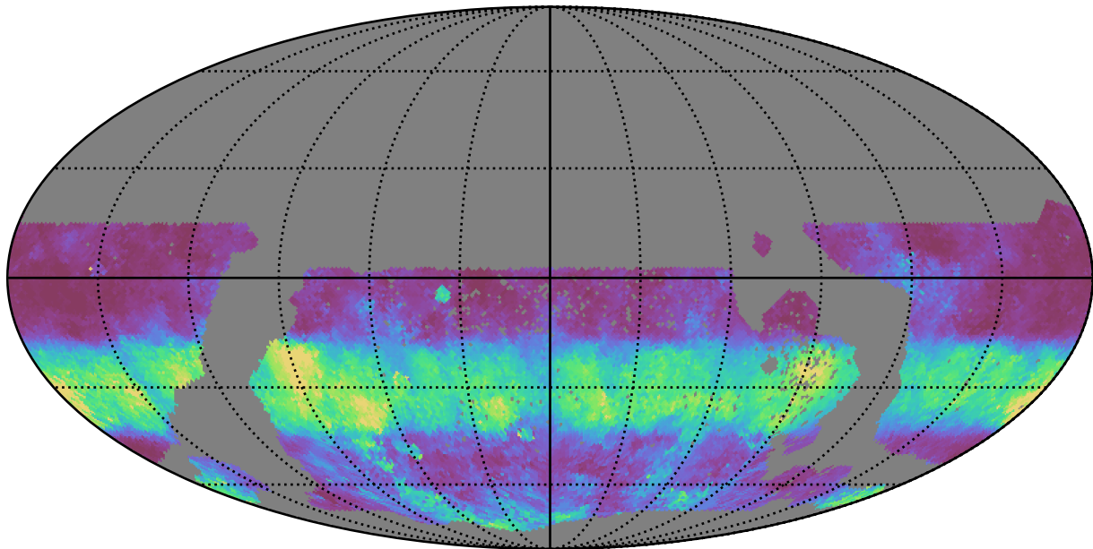
too_100_1v3.4_10yrs WFD g band: Median normairmass
