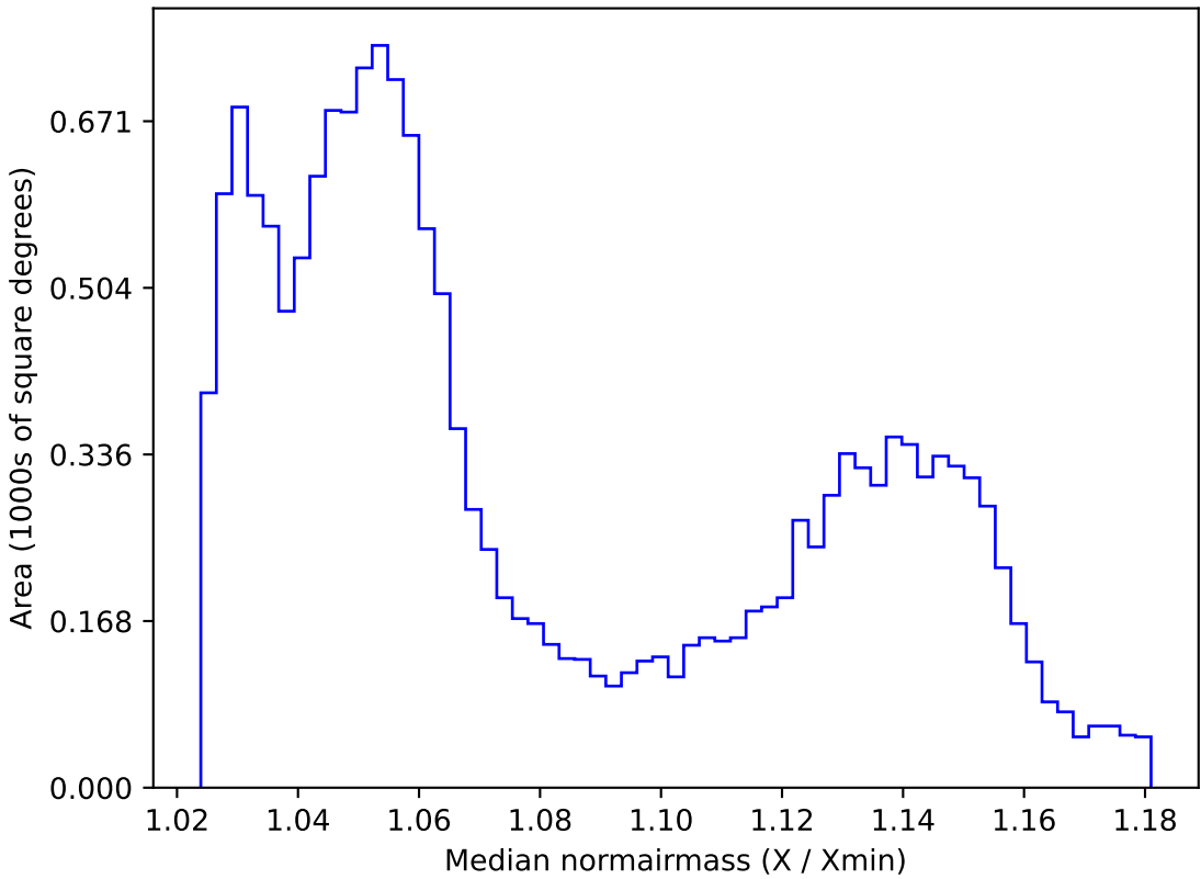
too_100_1v3.4_10yrs WFD all bands: Median normairmass
