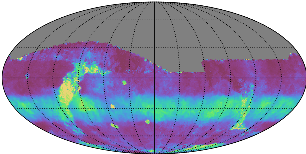
too_100_1v3.4_10yrs All sky z band: Median normairmass
