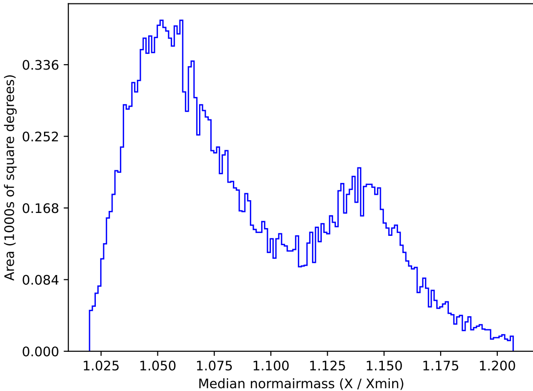
too_100_1v3.4_10yrs All sky y band: Median normairmass
