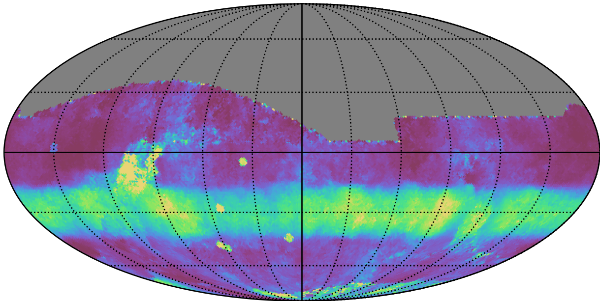
too_100_1v3.4_10yrs All sky r band: Median normairmass
