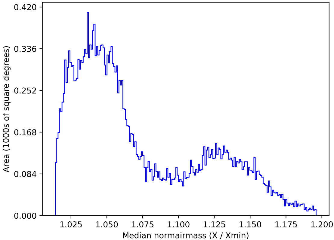
too_100_1v3.4_10yrs All sky r band: Median normairmass
