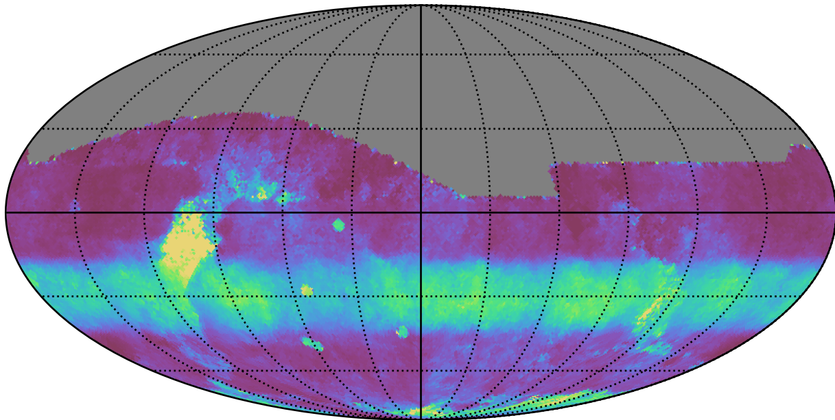
too_100_1v3.4_10yrs All sky i band: Median normairmass
