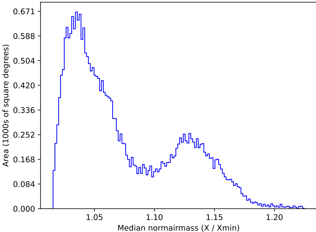
too_100_1v3.4_10yrs All sky i band: Median normairmass
