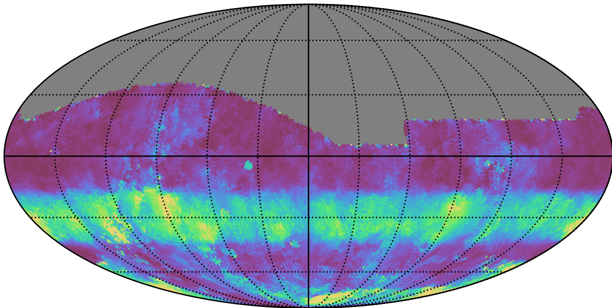
too_100_1v3.4_10yrs All sky g band: Median normairmass
