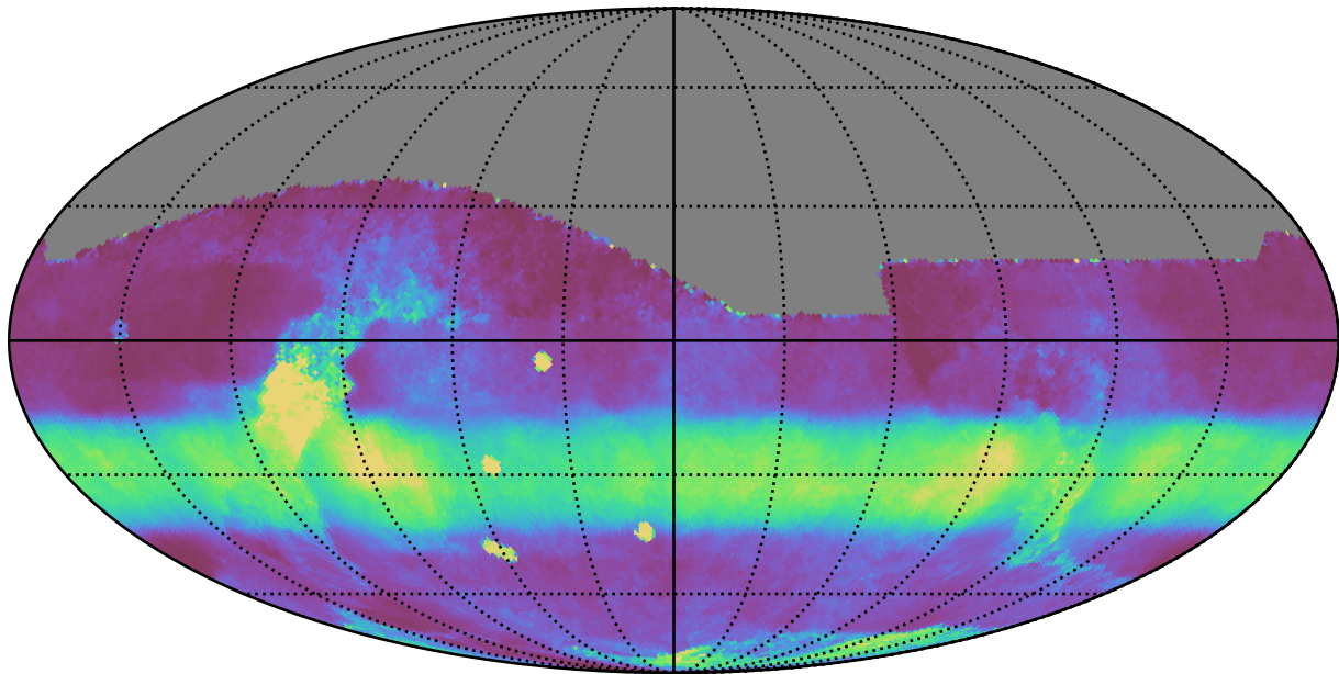
too_100_1v3.4_10yrs All sky all bands: Median normairmass
