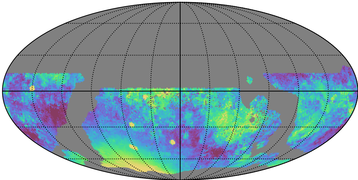
too_100_1v3.4_10yrs WFD z band: Median moonDistance
