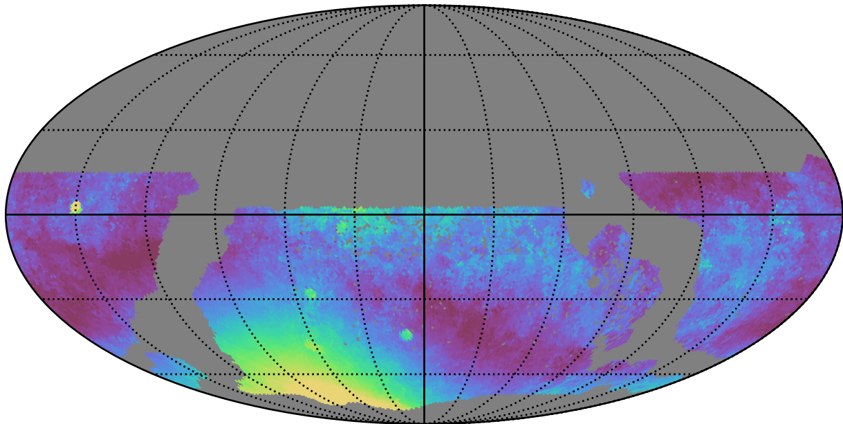
too_100_1v3.4_10yrs WFD y band: Median moonDistance
