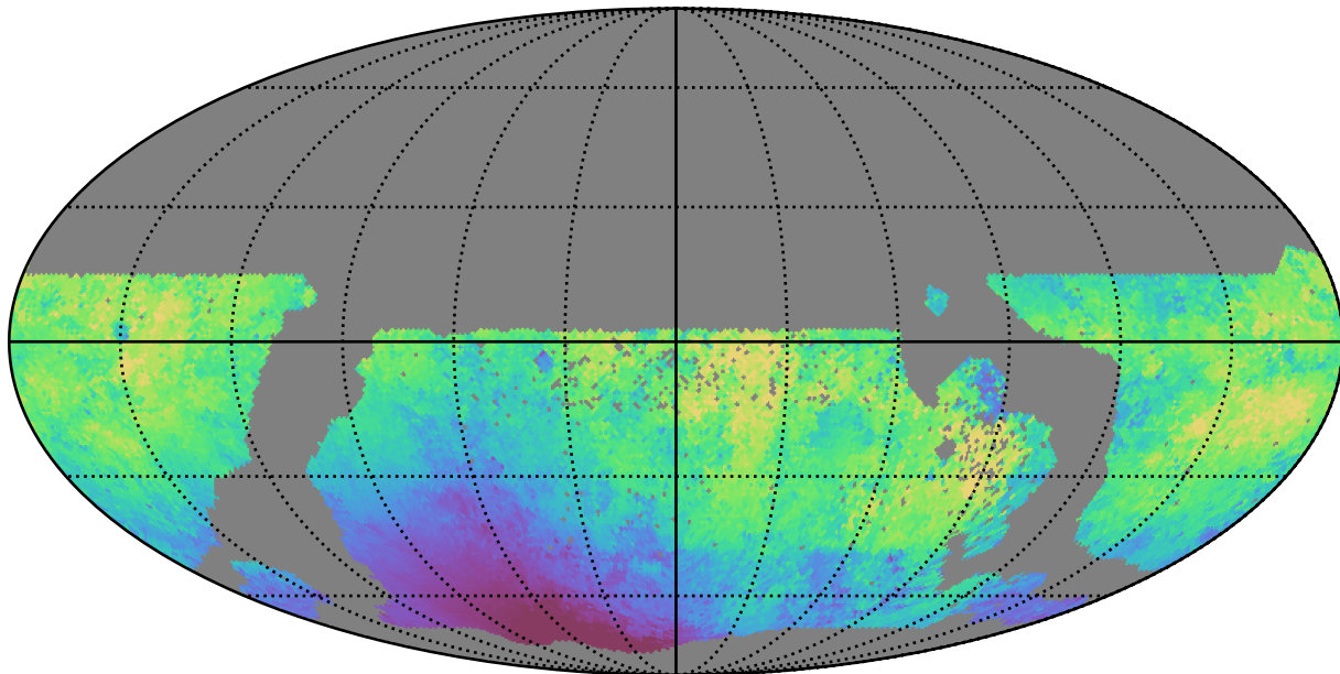
too_100_1v3.4_10yrs WFD u band: Median moonDistance
