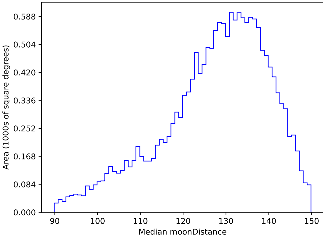
too_100_1v3.4_10yrs WFD u band: Median moonDistance
