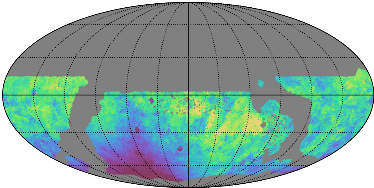
too_100_1v3.4_10yrs WFD r band: Median moonDistance
