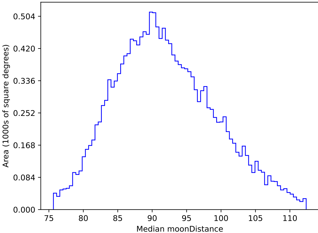
too_100_1v3.4_10yrs WFD i band: Median moonDistance
