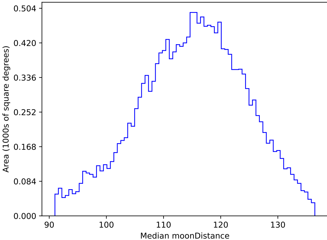
too_100_1v3.4_10yrs WFD g band: Median moonDistance
