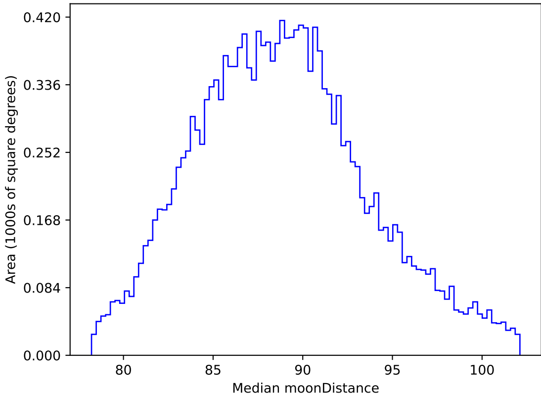
too_100_1v3.4_10yrs WFD all bands: Median moonDistance
