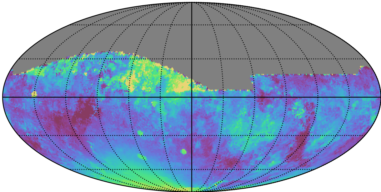
too_100_1v3.4_10yrs All sky z band: Median moonDistance
