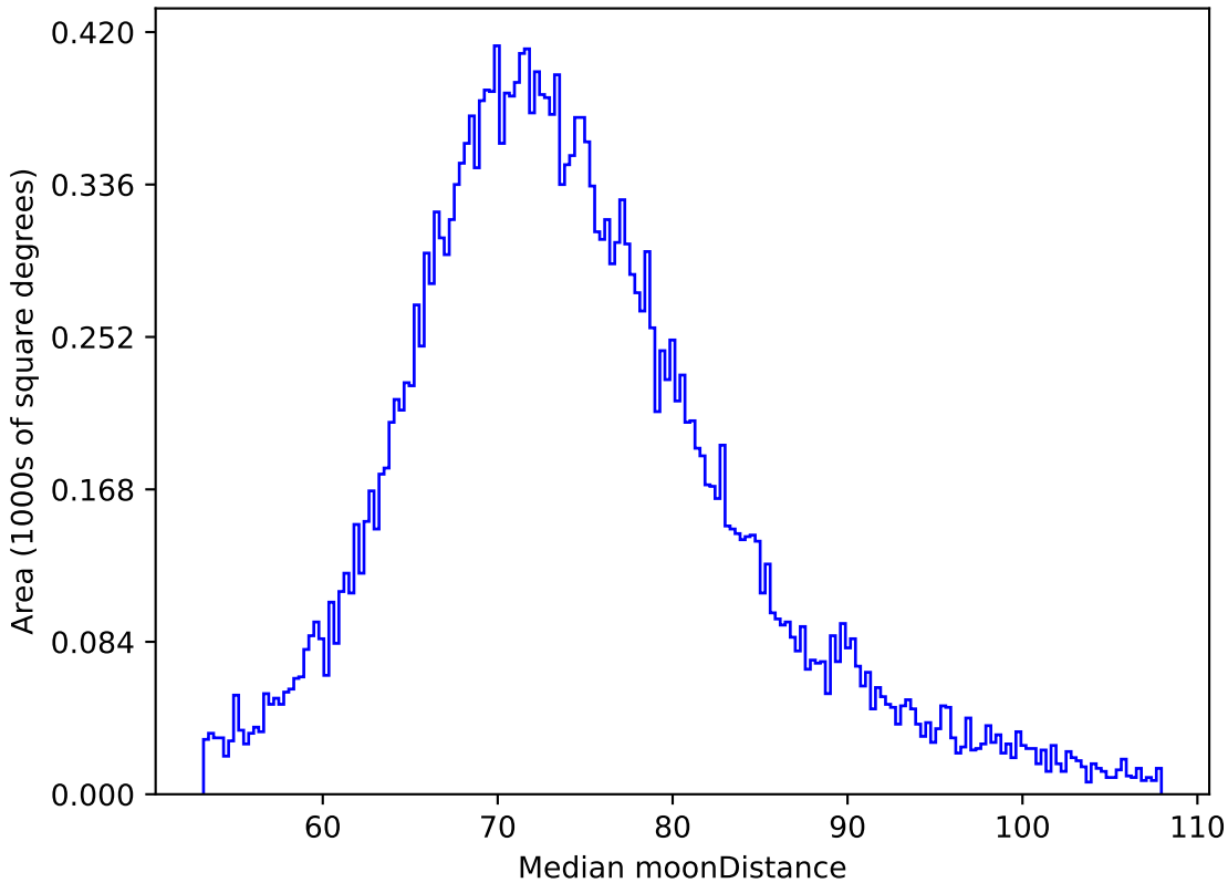
too_100_1v3.4_10yrs All sky z band: Median moonDistance
