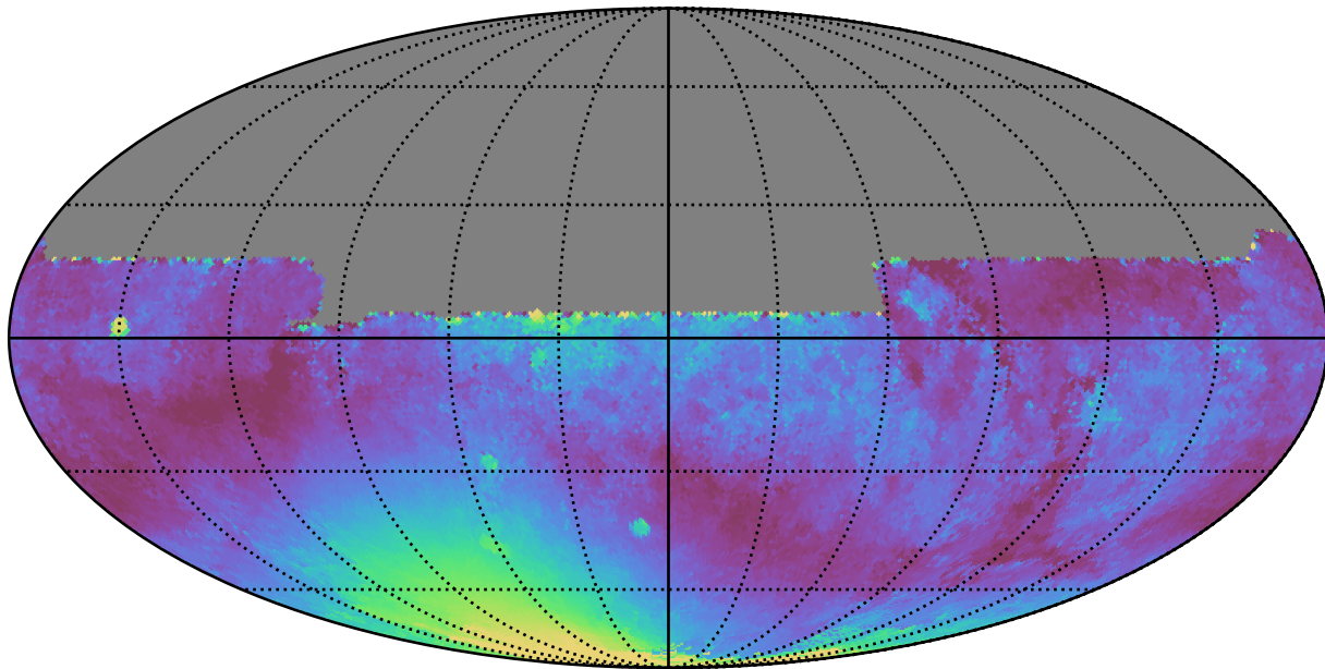
too_100_1v3.4_10yrs All sky y band: Median moonDistance
