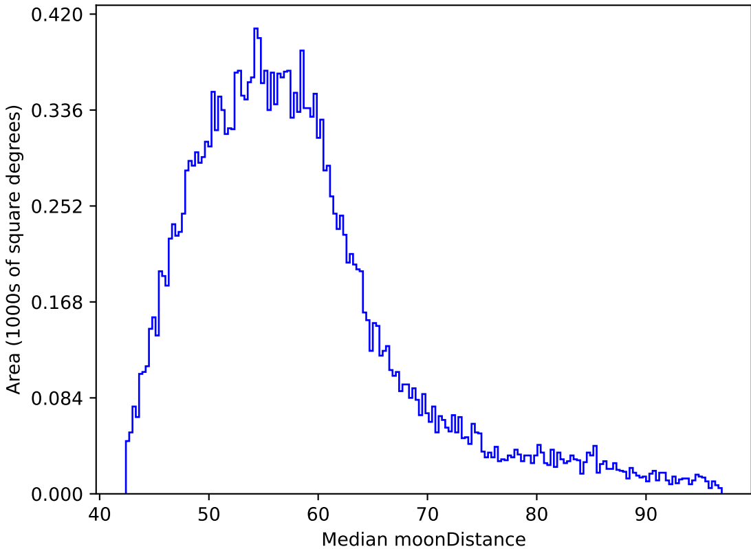
too_100_1v3.4_10yrs All sky y band: Median moonDistance
