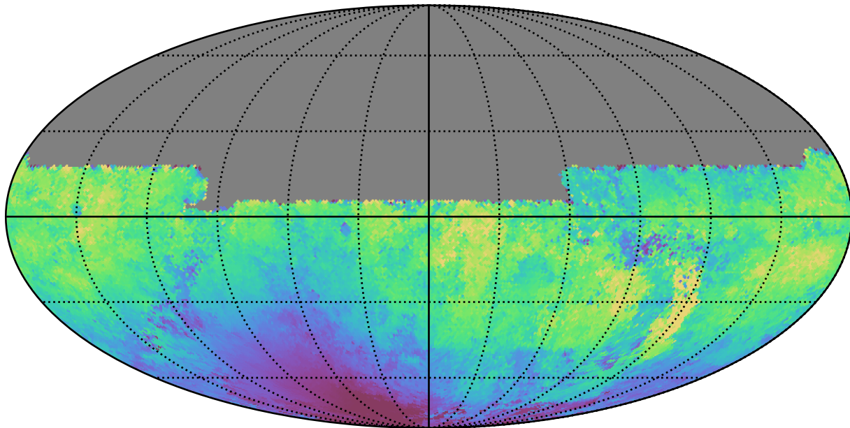
too_100_1v3.4_10yrs All sky u band: Median moonDistance
