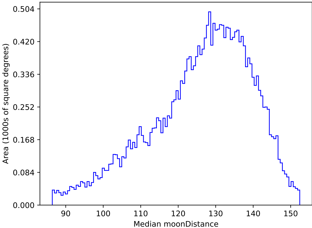
too_100_1v3.4_10yrs All sky u band: Median moonDistance
