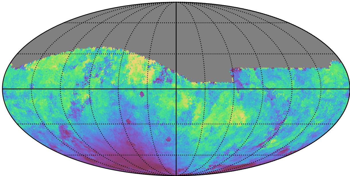
too_100_1v3.4_10yrs All sky r band: Median moonDistance
