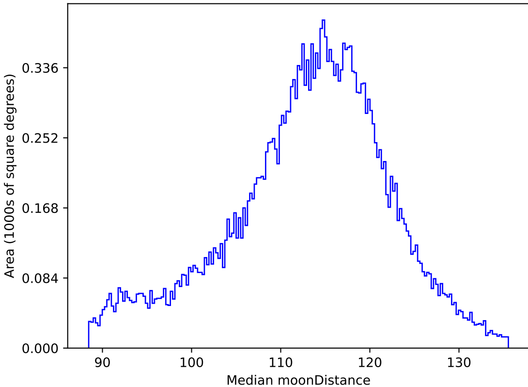
too_100_1v3.4_10yrs All sky r band: Median moonDistance
