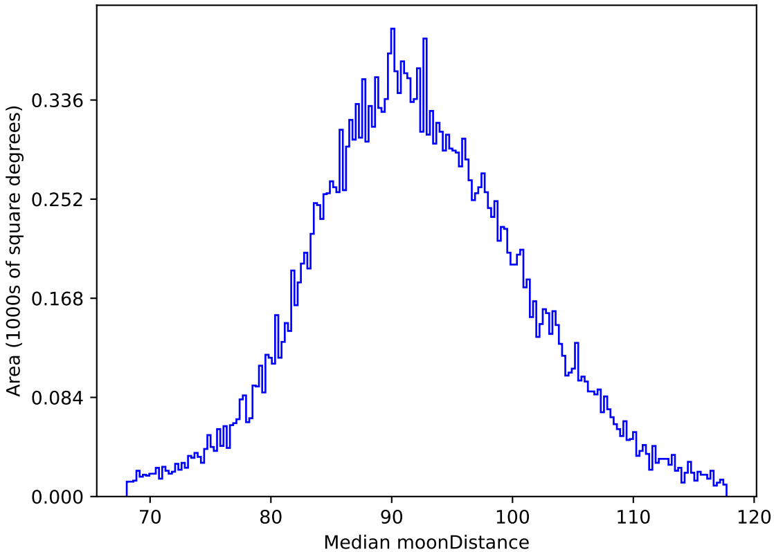
too_100_1v3.4_10yrs All sky i band: Median moonDistance
