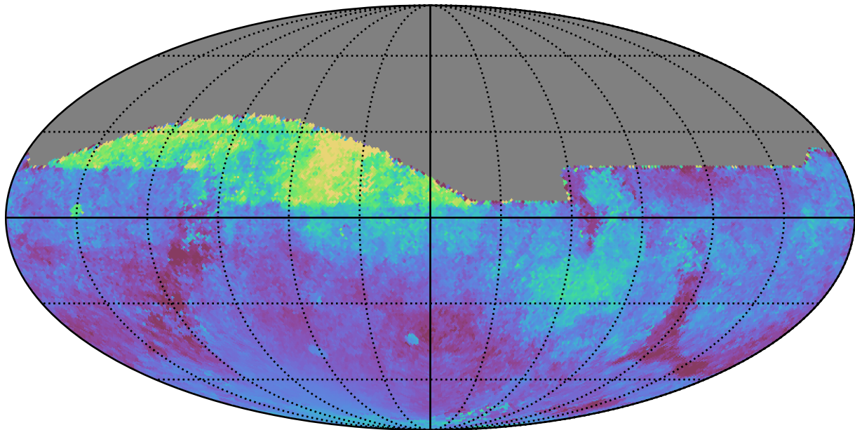
too_100_1v3.4_10yrs All sky all bands: Median moonDistance
