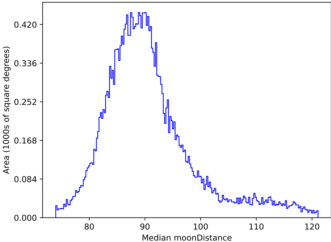
too_100_1v3.4_10yrs All sky all bands: Median moonDistance
