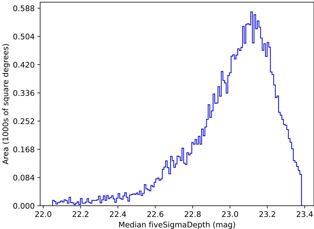
too_100_1v3.4_10yrs Yr 1 z band: Median fiveSigmaDepth
