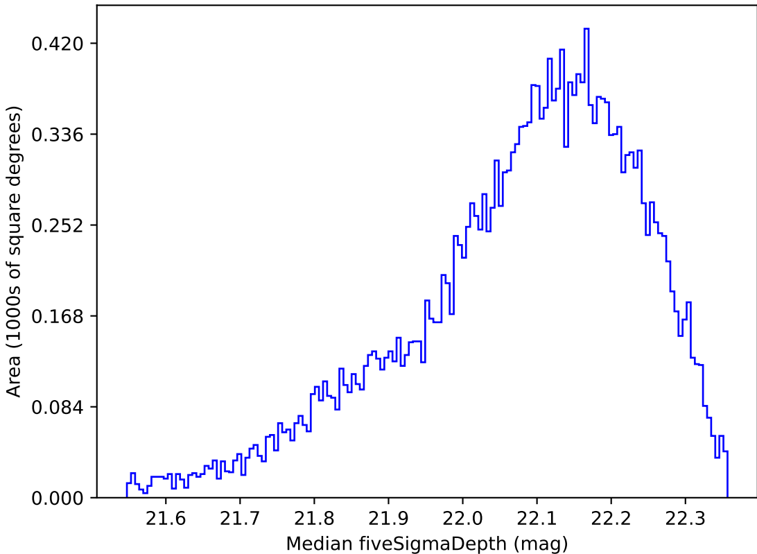
too_100_1v3.4_10yrs Yr 1 y band: Median fiveSigmaDepth
