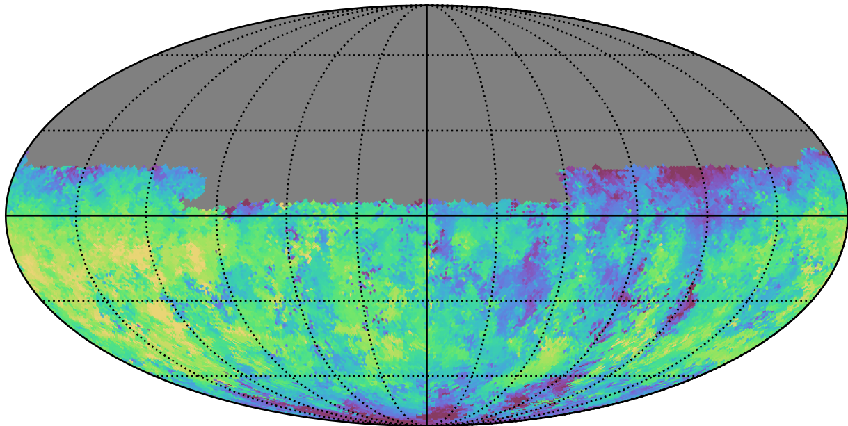
too_100_1v3.4_10yrs Yr 1 u band: Median fiveSigmaDepth
