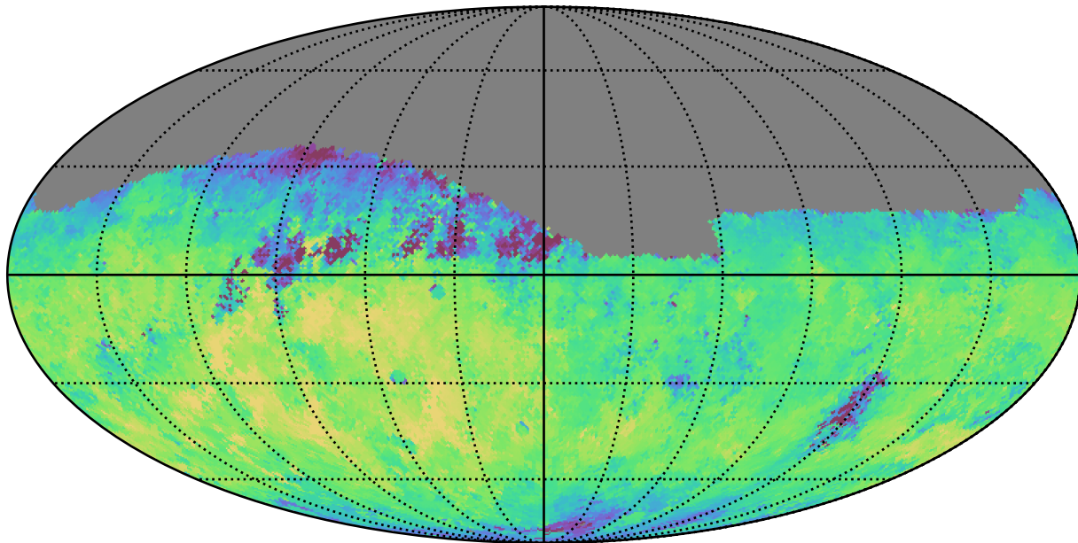
too_100_1v3.4_10yrs Yr 1 r band: Median fiveSigmaDepth
