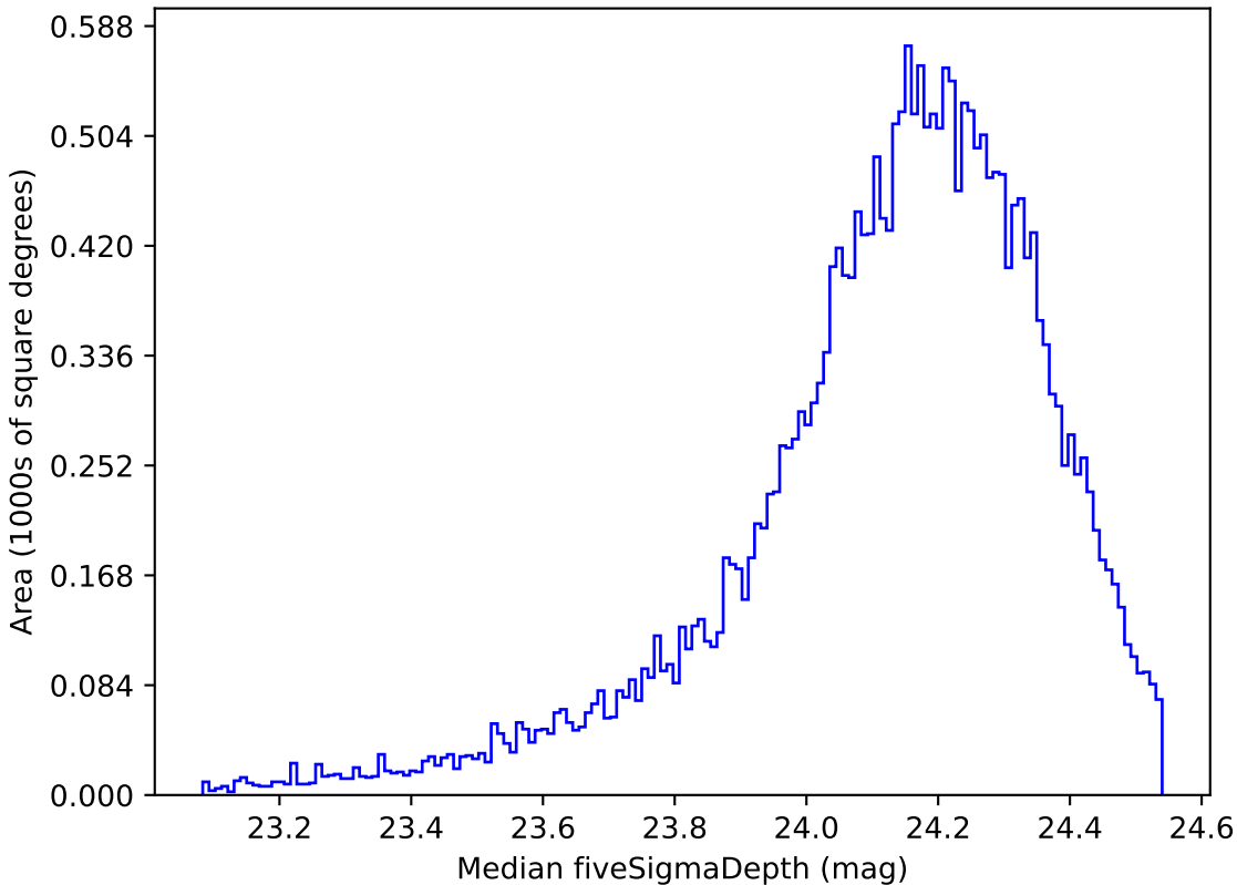
too_100_1v3.4_10yrs Yr 1 r band: Median fiveSigmaDepth
