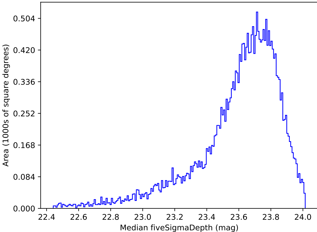
too_100_1v3.4_10yrs Yr 1 i band: Median fiveSigmaDepth
