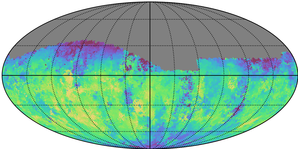
too_100_1v3.4_10yrs Yr 1 g band: Median fiveSigmaDepth
