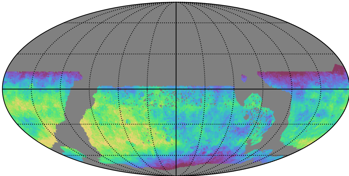
too_100_1v3.4_10yrs WFD z band: Median fiveSigmaDepth
