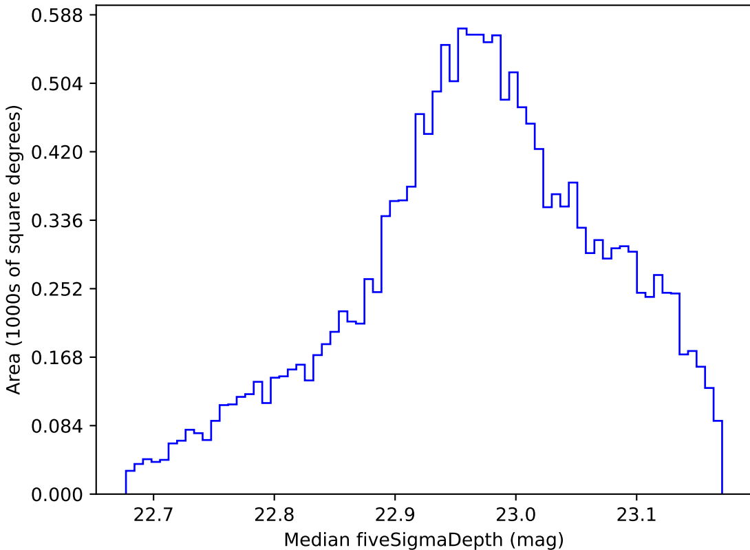
too_100_1v3.4_10yrs WFD z band: Median fiveSigmaDepth
