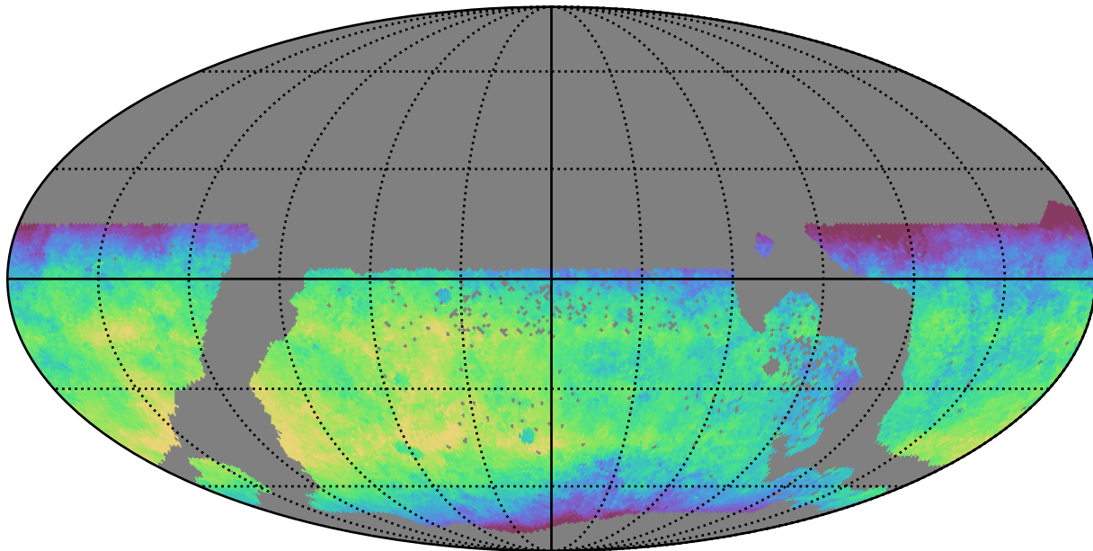
too_100_1v3.4_10yrs WFD y band: Median fiveSigmaDepth
