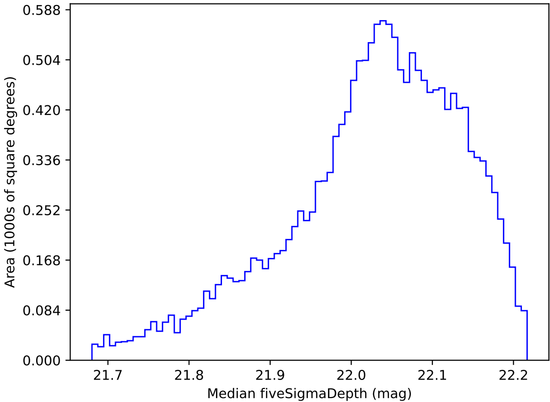
too_100_1v3.4_10yrs WFD y band: Median fiveSigmaDepth
