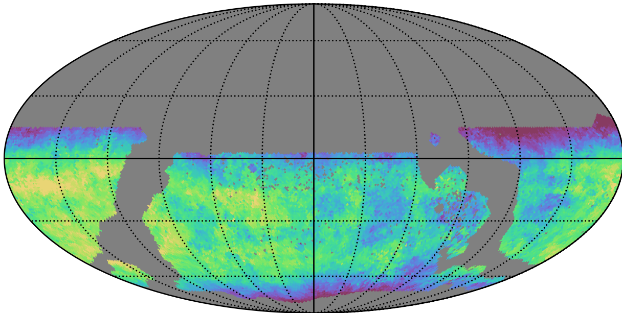
too_100_1v3.4_10yrs WFD u band: Median fiveSigmaDepth
