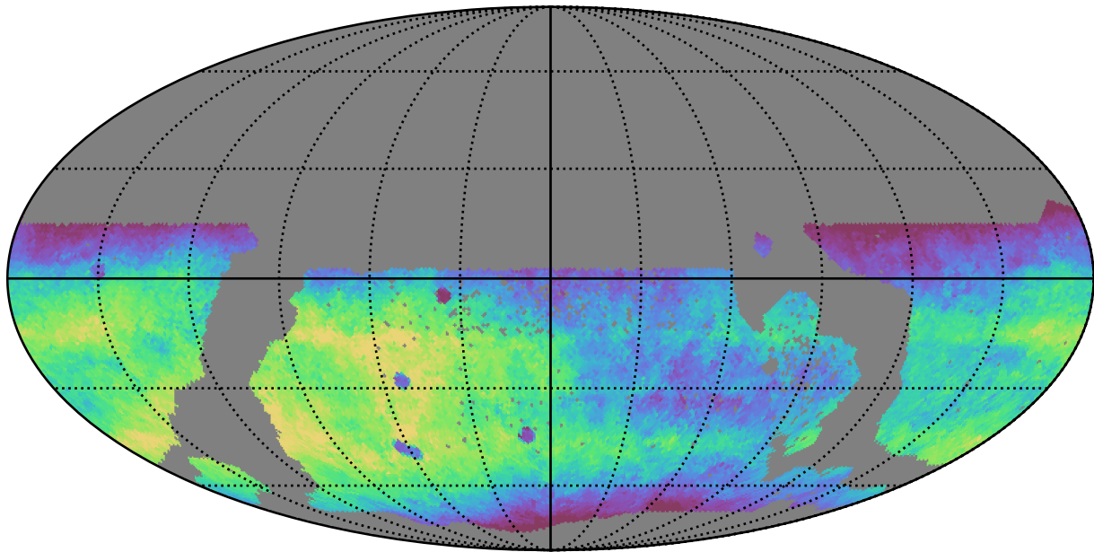
too_100_1v3.4_10yrs WFD r band: Median fiveSigmaDepth
