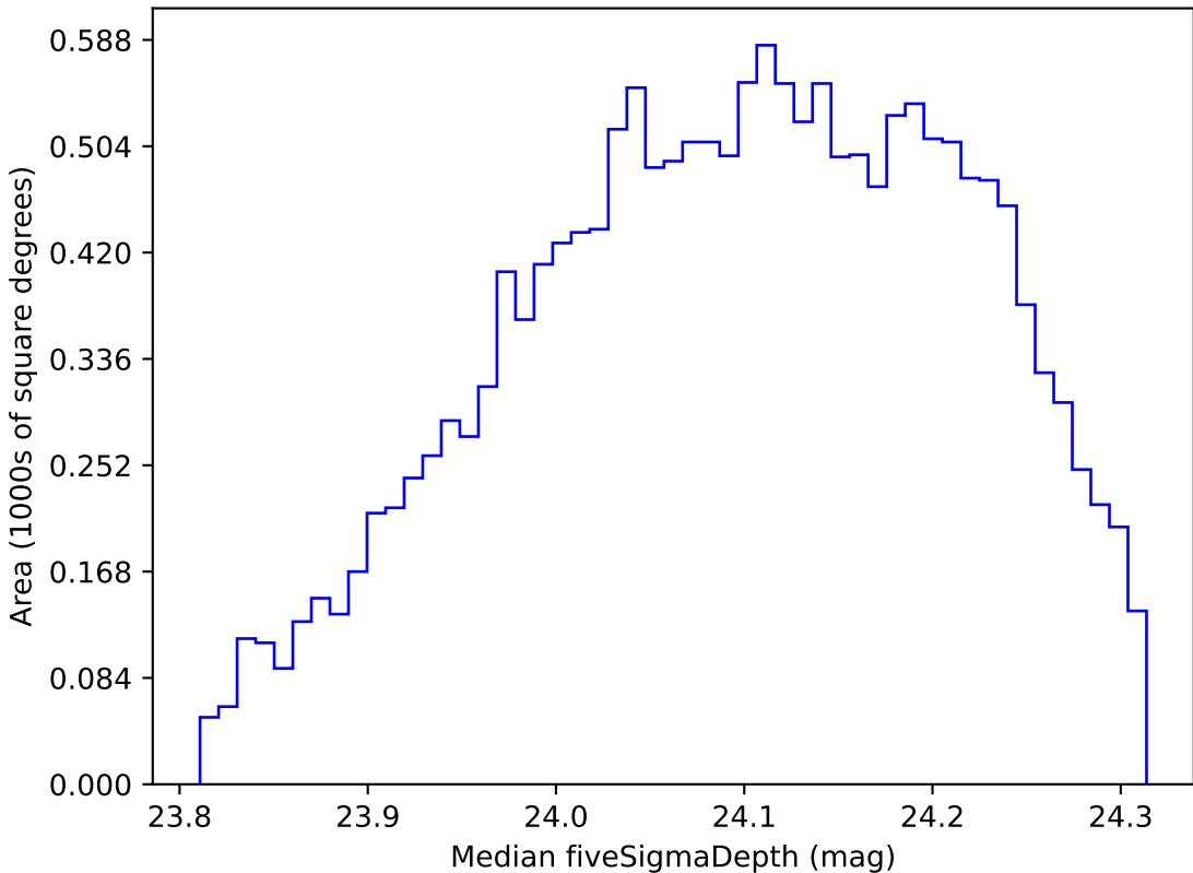
too_100_1v3.4_10yrs WFD r band: Median fiveSigmaDepth
